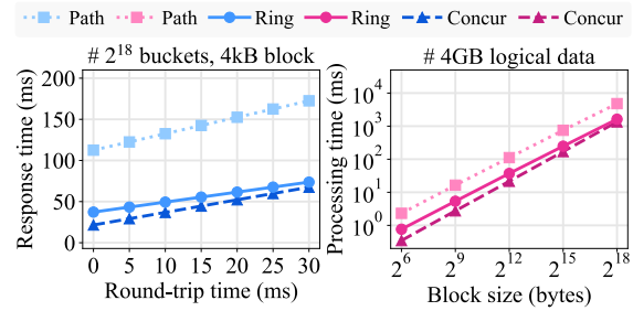
Figure 9: The performance of V-ORAM under realistic settings. We evaluate an V-ORAM with 4GB logical data under various RTT (Left) and block size (Right).
