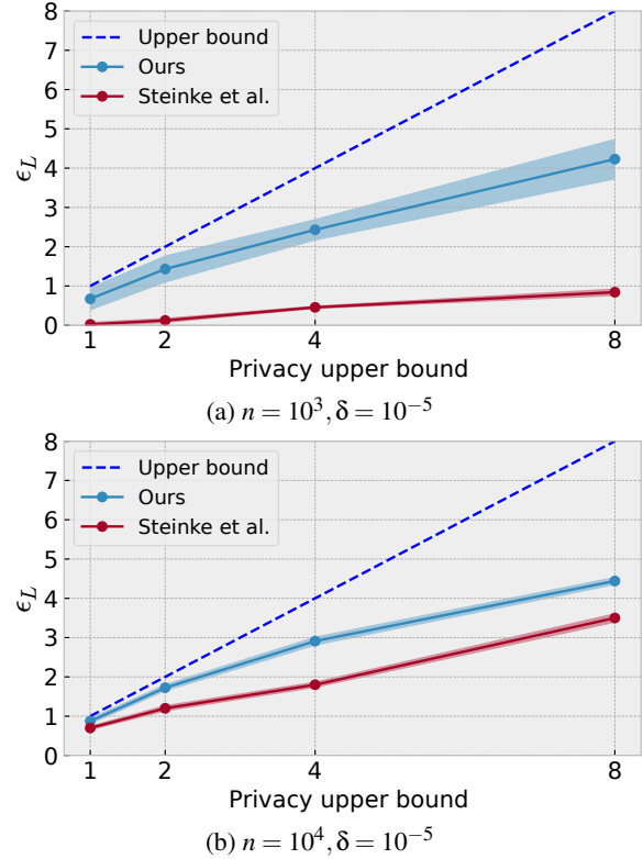
Figure 9: Privacy lower bounds for auditing DP-SGD at white-box setting. The experimental dataset is CIFAR10, the same as that in [37].
