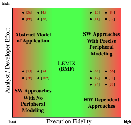
Figure 2: LEMIX in Contrast to Existing Rehosting Approaches.
