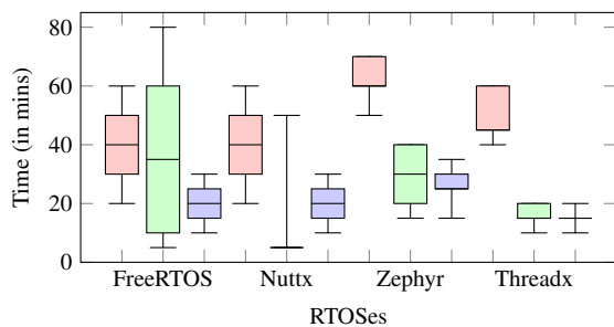
Figure 4: Comparison of manual effort time (y-axis) across RTOSes (x-axis), categorized into: (a) ■ - Preconfigurations and source modifications; (b) ■ - Non-automated compiler errors; and (c) ■ - Macro ASM adjustments.
