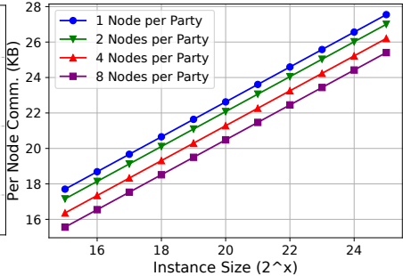
Figure 5: Comm. with RSS.
