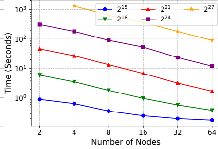
Figure 11: Public delegation scalability.
