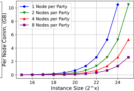
Figure 8: Comm. with AddSS.
