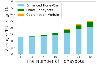
Figure 16: Resource consumption distribution
