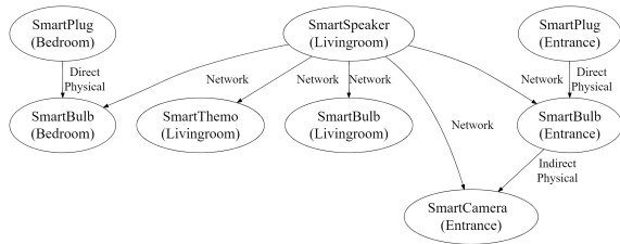
Figure 5: Dependency Graph Example
