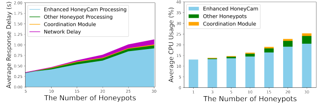
Figure 15: Response delay against one attack action
