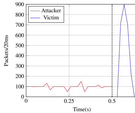
(a) Experiment with three hosts (2550 packets, 32 paths, sent in 0.50s, received in 0.078s).
