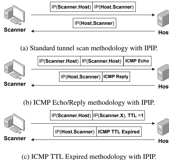
Figure 2: Illustration of the three main scan methodologies. The first arrow shows the scanner’s sent probe, while the second arrows show the host’s response.
