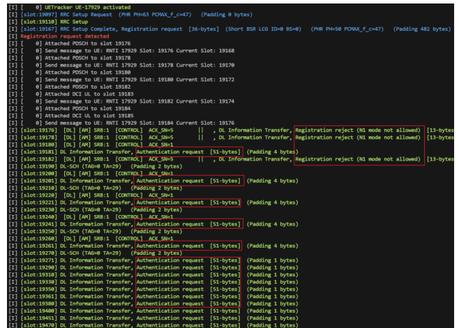
Figure 18: Registration Reject Example output
