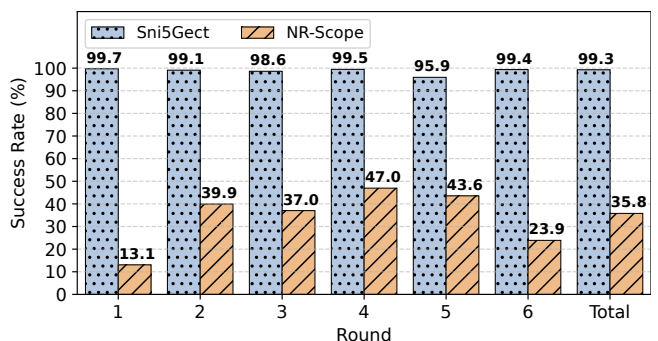
Figure 10: Success Rate of DCI search
