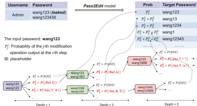
Figure 3: Example of generating reused passwords with beam search algorithm. Here, we suppose the original password is pw = \text{wang123} , and the beam width is k = 2 . The red P indicates the probability of the most feasible k valid modification operations in each round (the product of the probability from the root to the current node), and the dotted arrow indicates the process of summarizing the paths to get the final password guess set.
