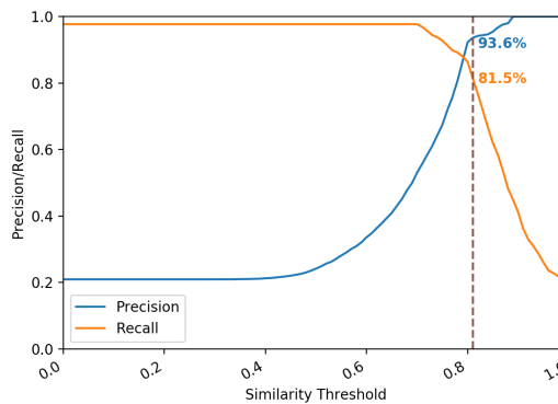
Figure 9: Precision and recall of identifying IoT data items with different similarity thresholds.
