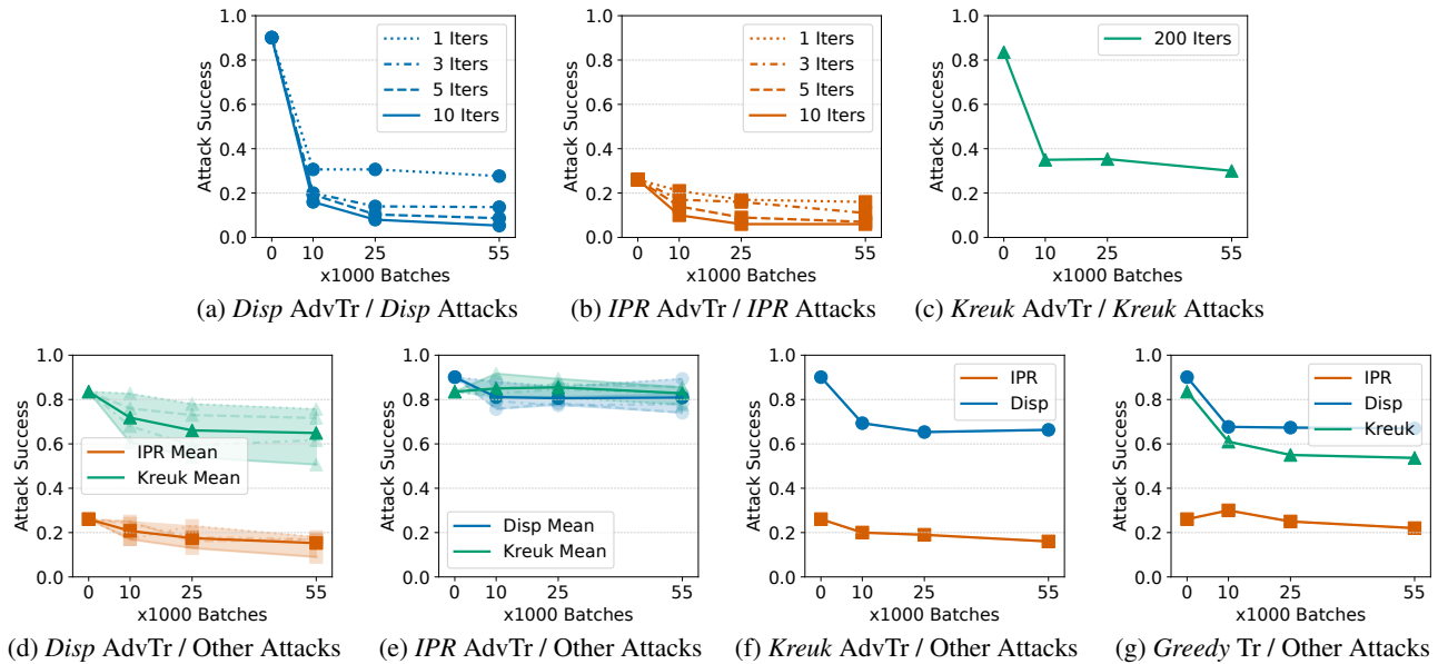
Figure 3: Comparing attack success rates for Disp , IPR , and Kreuk attacks up to 200 iterations between models trained with varying number of adversarial examples and training attack iterations. Training on these attacks substantially increases model robustness to the same attack, as shown in Figs. 3a–3c. The downward trends in Fig. 3d and Fig. 3f show that training on Disp or Kreuk attacks reduces model vulnerability to other attacks by a smaller amount. “{ IPR , Disp , Kreuk } Mean” is the mean attack success rate over multiple adversarially trained models (e.g., 1-, 3-, 5-, 10-iteration Disp -adversarially-trained models in Fig. 3d).
