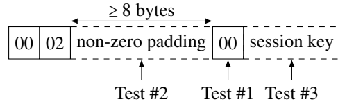
Figure 2: PKCS#1 v1.5 padding. Test #1-#3 mark the boolean tests identified by Bardou et al.
