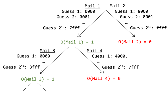
Figure 4: Empty Line Oracle: Batching multiple oracle queries to perform a binary search of the first two bytes of a block. The guesses of each mail are in a single message part.
