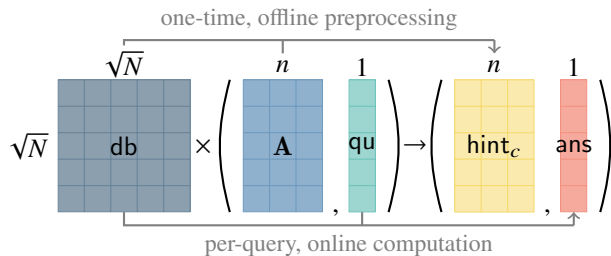
Figure 3: The server computation in SimplePIR. Each cell represents a \mathbb{Z}_q element, and \times denotes matrix multiplication. The server performs the bulk of its work in a one-time preprocessing step. Thereafter, the server can answer each client’s query with a lightweight online phase.
