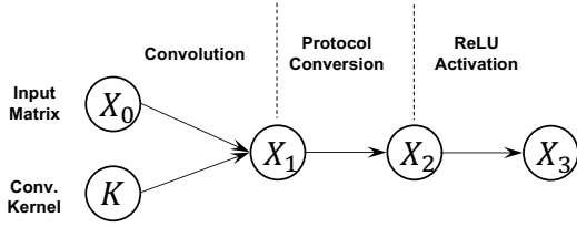
Figure 6: Dependency graph generated from a convolution followed by ReLU activation.
