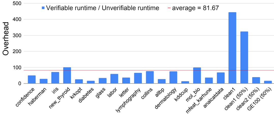
FIGURE 13—Overhead of Otti’s prover (proof and solve) for training and proving a perceptron using SGD versus a baseline that lacks proofs.
