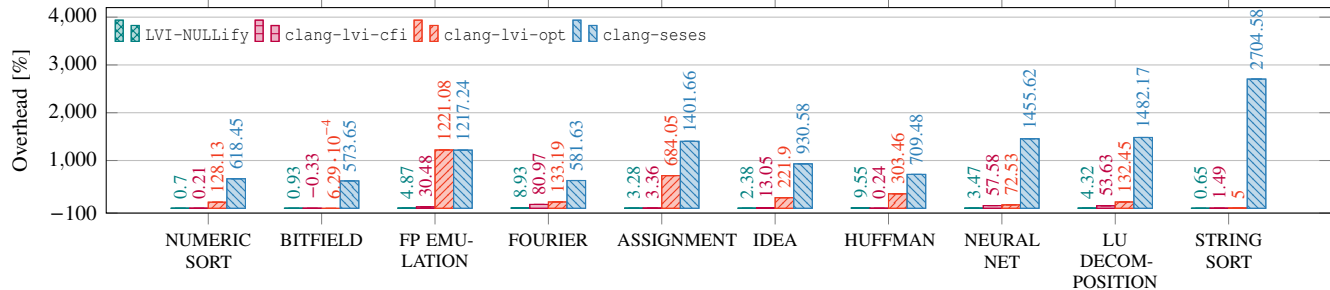
Figure 4: Mean runtime overhead in sgx-nbench [58] on our i5-10210U@1.6GHz of LVI-NULlify vs. Intel’s control-flow and optimized-cut mitigations as well as SESES. N=50, standard deviations vs unmitigated mean plotted, but too small to be visible.
