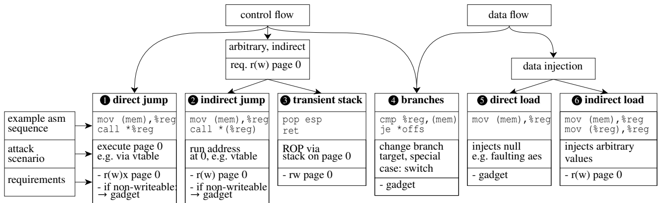
Figure 1: Categorization of LVI-NUL into control-flow and data-flow attacks. Subcategories list the different attack vectors and example assembly sequences for each (in AT&T syntax), the attack scenario, and their requirements.
