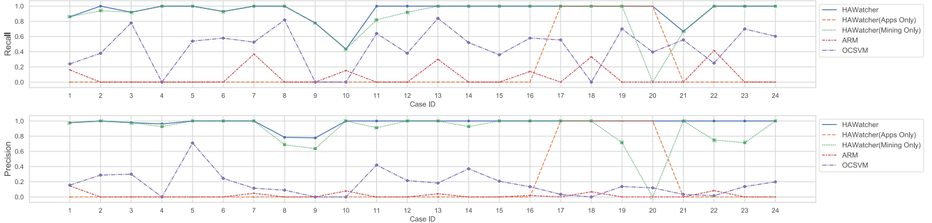
Figure 8: Recall and precision of HAWatcher and four other detectors for comparison purposes.
