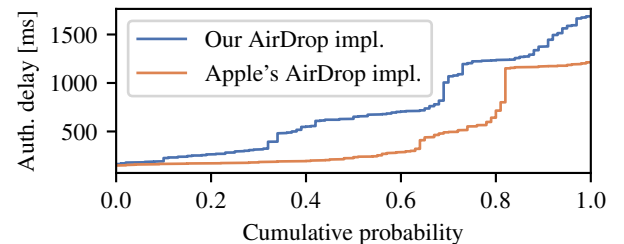
Figure 11: Authentication delay of our AirDrop implementation and Apple’s (MacBook Pro 2019 → iPhone 12 via AWDL).
