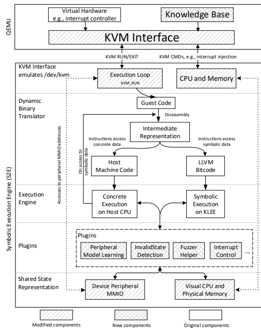
Figure 2: Architecture of \mu Emu
