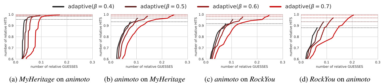
Figure 4: Effect of the parameter \beta on the guessing performance for four different combinations of password sets and PasswordPro rules. Plots are normalized according to the results of the standard mangling rules attack (i.e., \beta = 1 ). For instance, (x=0.1, y=0.95) means that we guessed 95% of the password guessed with the standard mangling rules attack by performing 10% of the guesses required from the latter.
