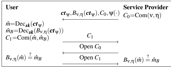
Figure 3: Release protocol for a computed value \hat{m} .
