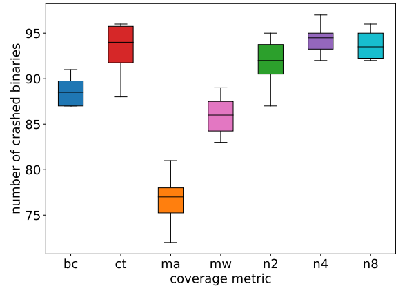
Figure 3: Number of crashed CGC binaries. Because each binary only has one vulnerability, this number is equivalent to the total number of unique crashes.
