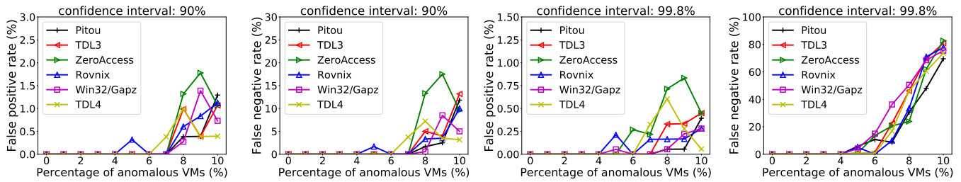
Figure 6: Autoencoder performance, with 90% and 99.8% confidence intervals, for different types of Windows kernel malware and rates of infection in a herd of 100 VMs. Points represent averages over twenty trials.
