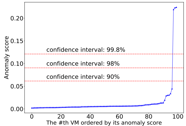
Figure 5: Error scores from the autoencoder-based analysis of an example herd of 100 VMs, three of which are infected with malware. The scores of the infected VMs (upper right) are flagged because they exceed a threshold, as determined by a confidence interval.
