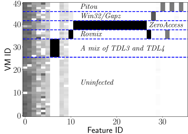
Figure 4: Similarity matrix for an experiment involving 50 VMs running Windows, many infected with malware. In this visualization, higher similarity scores have lighter colors.
