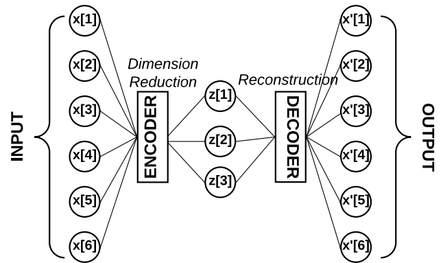
Figure 2: Autoencoder architecture.
