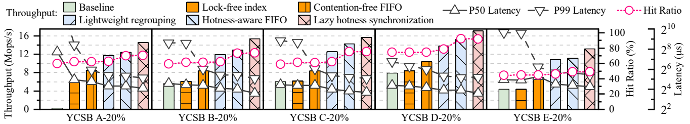
Figure 18: Performance contributions of different techniques across YCSB workloads at 20% cache sizes.
