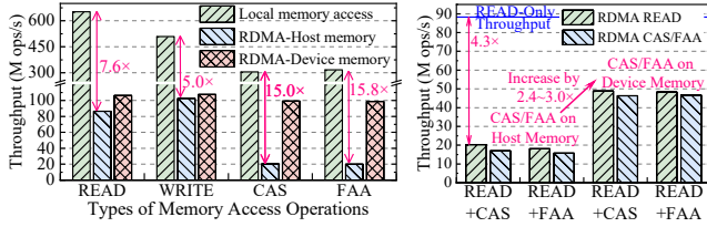
(a) Performance: Local memory access (b) Performance interference vs. RDMA in Host/Device memory between RDMA verbs
