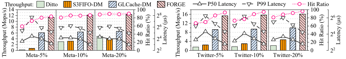
Figure 15: Throughputs, latencies, and hit ratios in real-world workloads at 5%, 10%, 20% cache sizes with variable object sizes.
