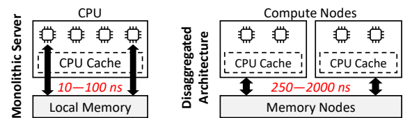
Figure 1: Memory access latencies in different architectures.
