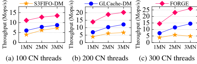
Figure 16: The scalability of systems with CNs and MNs in the Meta workload at 20% cache sizes.
