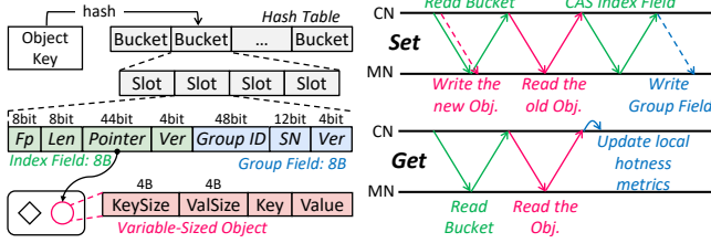
Figure 6: The data structures of the hash table and object.
