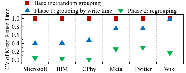
Figure 5: Similarity of objects grouped by different schemes.
