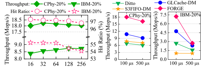
Figure 17: The sensitivity analysis of system performance.
