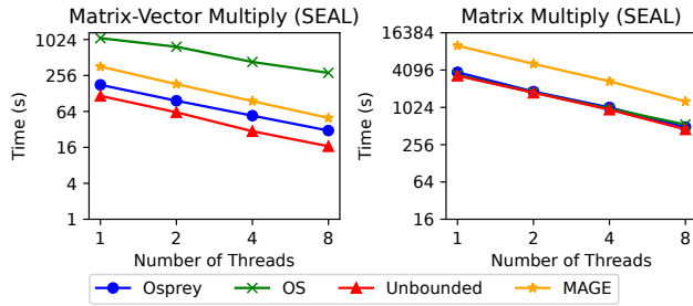
Figure 8: Multithreaded performance.
