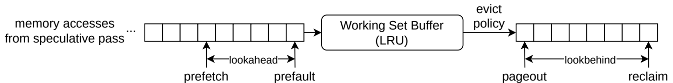
Figure 4: Workflow for Osprey's programmed pass. Each box represents a batch of memory accesses.
