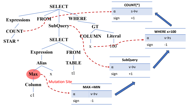
Figure 4: Example of how the proposed algorithm propagates local semantic changes across the SQL AST.
