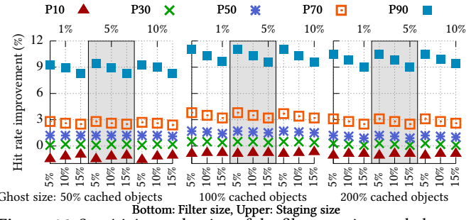
Figure 16: Sensitivity evaluation of the filter, staging, and ghost queue sizes (%). The filter queue ranges 5%, 10%, and 15%; the staging queue is set to 1%, 5%, and 10%; and the ghost queue varies across 50%, 100%, and 200% of the cache size. Cache size is 10% of WSS
