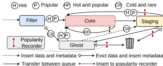
Figure 8: An overview of MERLIN's key components and workflow.
