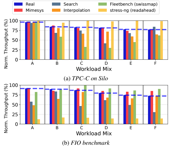
Figure 7: Application performance degradation while varying colocated workload mixes for (a) TPC-C on Silo and (b) FIO.
