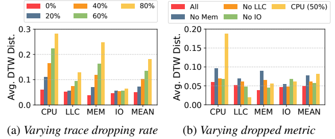
Figure 12: Sensitivity to input trace variations.
