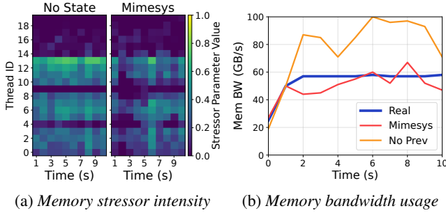
Figure 11: Effectiveness of state-aware conditioning.
