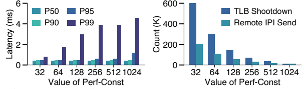
Figure 11: Tuning NR_MAX_BATCHED_MIGRATION to reduce tail latency, which requires understanding TLB shutdown behavior.
