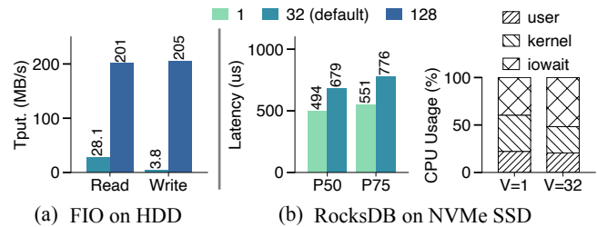
Figure 1: Performance benefits of changing the value of a perf-const BLK_MAX_REQUEST_COUNT based on hardware devices and workloads. The default value is 32.
