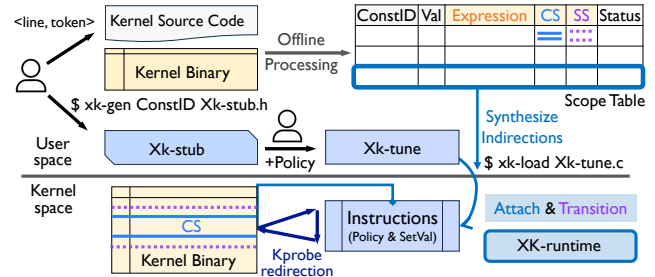
Figure 2: Overview of Xkernel.
