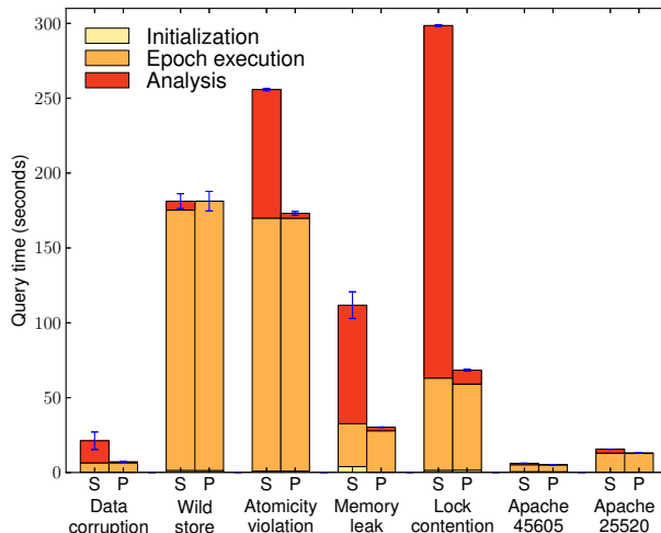
Figure 8: Analysis. We compare query time with sequential (S) and parallel (P) analysis using 64 cores. The regions in each bar show how much time is spent in each phase along the critical path of query processing.
