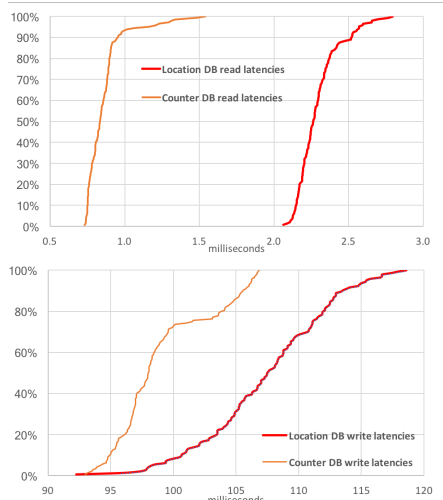
Figure 8: Distribution of client-side latencies for accessing the Akkio location and counter databases, (not taking the cache into account). Read latencies are shown in the top graph; write latencies in the bottom graph.
