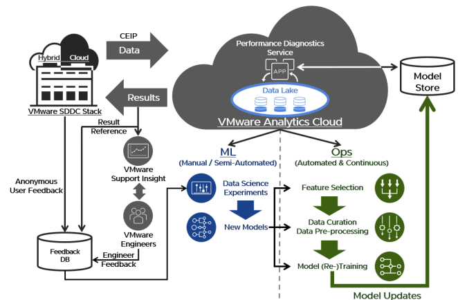
Figure 1. ML/Ops Lifecycle of Our Solution
