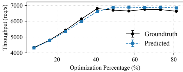
Fig. 3: Profiling results from SLOWPOKE for the Cart service in OnlineBoutique with mixed types of user requests. The x-axis is the percentage of optimization applied to Cart service, e.g., 50% optimization means a 50% reduction in average execution time per request. The y-axis is the end-to-end application throughput.
