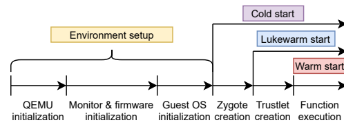
Figure 4: WALLET invocation phases.
