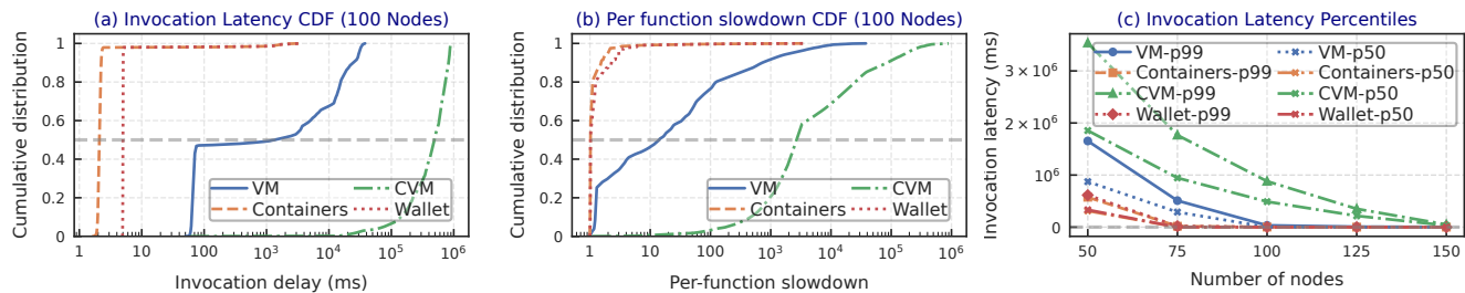
Figure 10: Scale-out results using Azure Functions production traces [142, 165].
