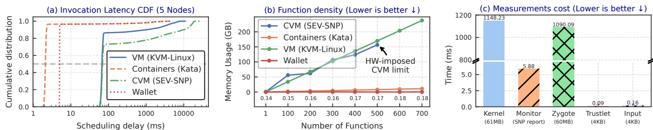
Figure 2: Serverless requirement analysis: (a) the scheduling delay, (b) the function density, and (c) attestation measurements.
