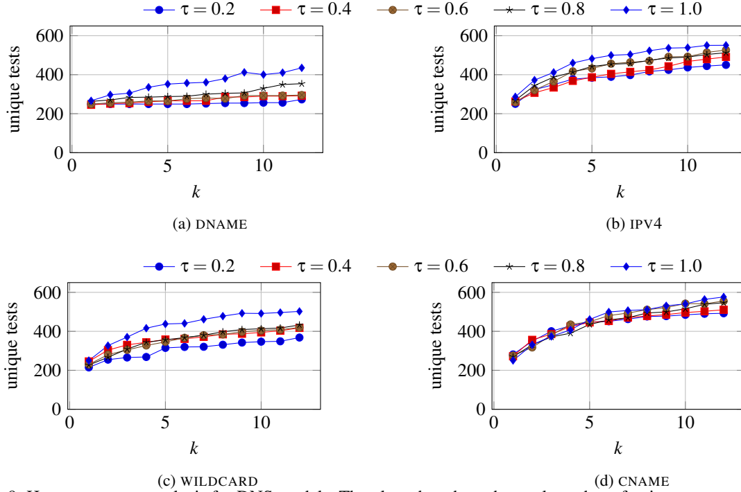
Figure 9: Hyperparameter analysis for DNS models. The plots show how the total number of unique tests vary as we increase the number of runs for different models.
