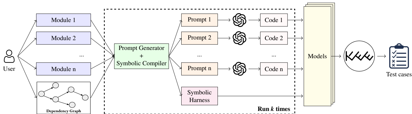
Figure 3: Architecture of EYWA. It takes modules and dependencies and produces k different protocol models.
