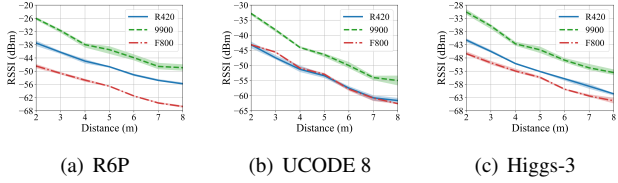
Figure 13: RSSI with respect to the reader-to-tag distance.
