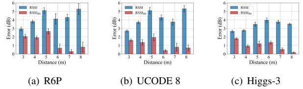
Figure 15: Correction error with respect to the distance.
