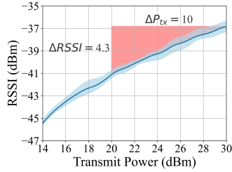
Figure 1: RSSI with respect to the transmit power.
