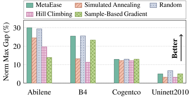
Figure 20: MetaEase delivers top-2 gaps compared to black-box searches when we analyze the example heuristic in §2.
