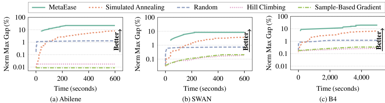
Figure 9: MetaEase finds larger performance gaps faster compared to black-box approaches. For a fair comparison, we allow all methods to fully utilize all threads available on the machine.
