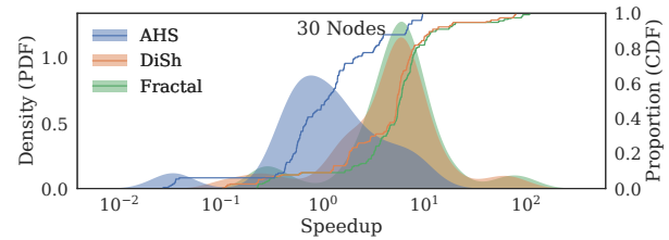
Fig. 4: Fault-free performance summary. Summary of AHS, DiSH, and FRACTAL 30-node fault-free speedups over Bash across all benchmarks: FRACTAL is comparable to DiSH and significantly faster than AHS.
