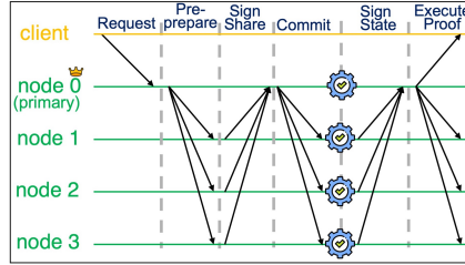
Figure 18: SBFT
