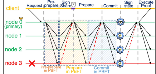
Figure 19: SBFT slow path (Linear PBFT)
