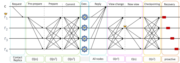
Figure 3: Different stages of PBFT protocol
