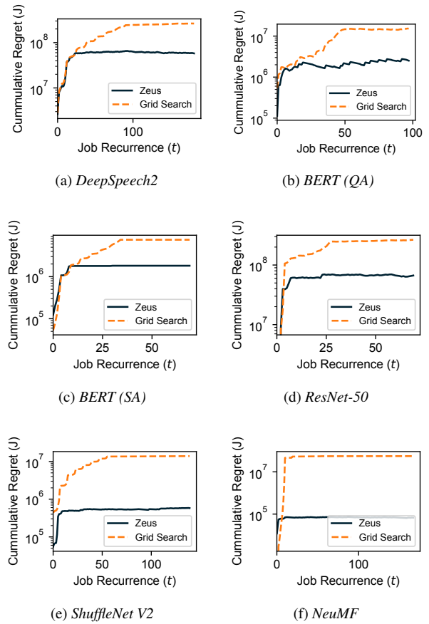
Figure 19: Cumulative regret of Zeus vs. Grid Search across all workloads.
