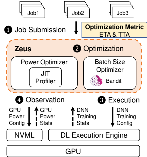
Figure 3: Zeus Workflow.
