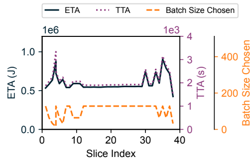
Figure 10: Energy and time consumption of training BERT with Zeus on Capriccio and the batch size chosen for each slice.
