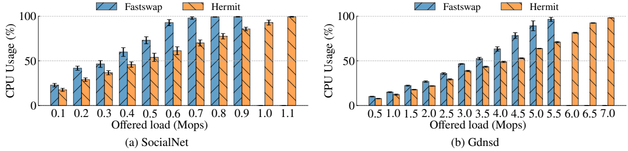
Figure 19: For SocialNet and Gdnzd, Hermit still saves 10%–40% CPU cycles under varying load compared with Fastswap, which is the key enabler it can achieve low tail latency under high load.
