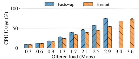
Figure 17: Hermit saves \sim 30% CPU cycles under varying load compared with Fastswap, which is the key enabler to achieve low 99 th percentile latency under high load.
