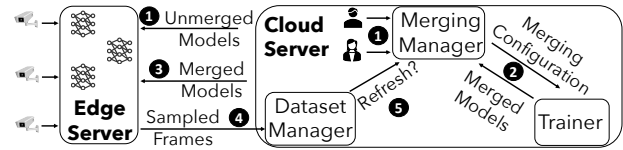
Figure 9: Gemel architecture.
