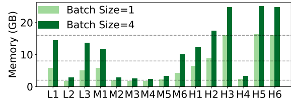
Figure 2: Per-workload memory requirements for two popular batch sizes used in video analytics [94]. Dashed lines represent the available GPU memory on several commercial edge boxes.
