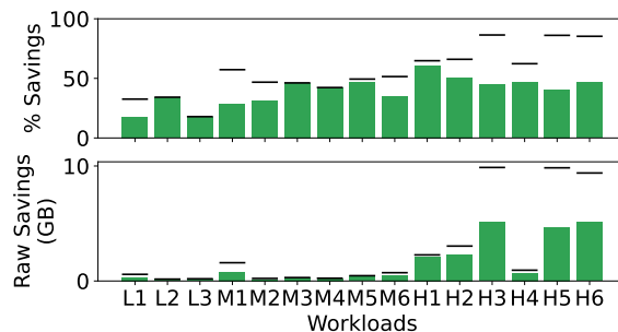
Figure 12: Gemel’s per-workload memory savings. Lines above bars show the theoretical optimal savings from Figure 6.
