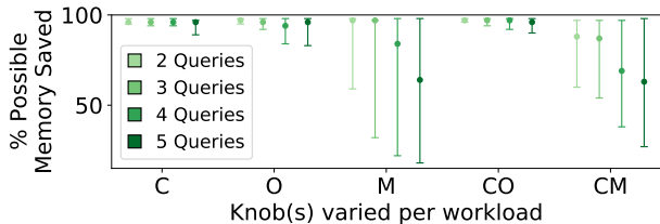
Figure 17: Memory savings across subset of generalization workloads, organized by workload size (color) and knobs varied (Camera, Object, Model). Distributions show median and 25-75% ile; accuracy target was 95%. Figure 22 has full graph.
