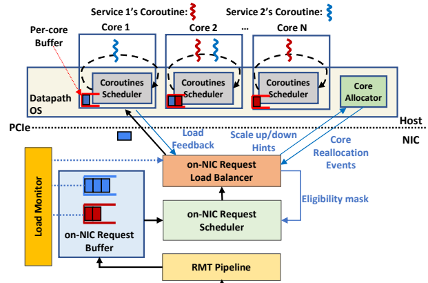
Figure 4: RingLeader Design.
