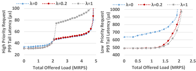
(a) High Priority Request's P99 tail latency (b) Low Priority Request's P99 tail latency Figure 14: JBSRQ's performance under different \lambda .
