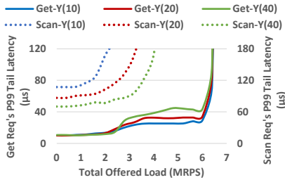
Figure 10: RocksDB performance.
