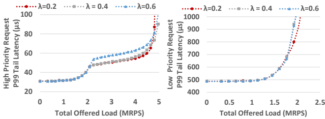
(a) High Priority Request's P99 tail latency (b) Low Priority Request's P99 tail latency Figure 15: JBSRQ's performance under different \lambda ( 0 < \lambda < 1 ).
