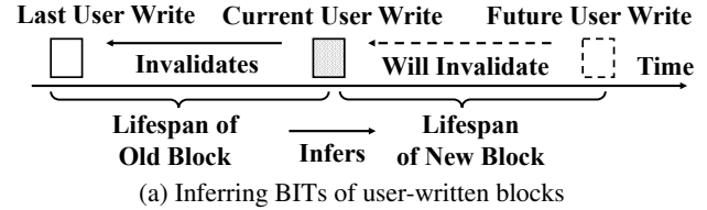
(a) Inferring BITs of user-written blocks
