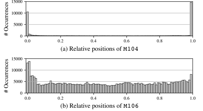
Figure 7: Histograms of the positions where M104 and M106 are used over all files.
