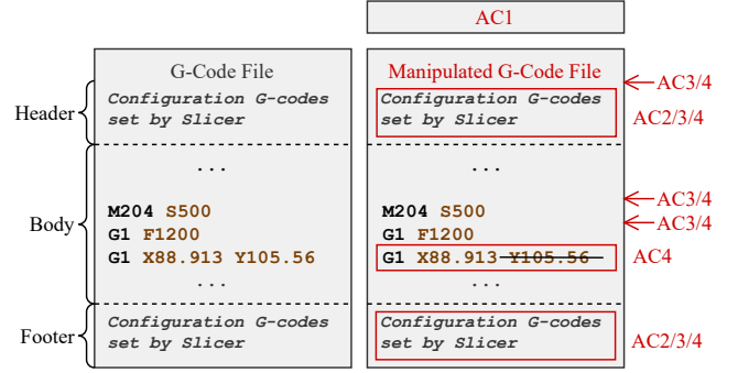
Figure 4: Depending on the AC, the attacker can manipulate the entire G-Code file (of a target print) or only parts of it. The file does not have to exist as such on the printer; it could be transferred interactively. AC2 can influence G-Codes in the header and footer (defined by the slicer). AC3 can inject G-Codes while the file is printing. AC4, the strongest attacker, can modify any content.
