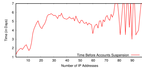
Figure 1: Average time (in days) before a spamming account was suspended in L , given the number of IP addresses accessing that account.
