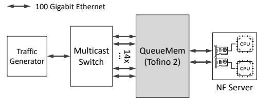
Figure 14: QUEUE-MEM testbed.
