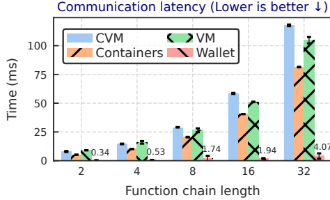
Figure 9: Latencies of function chains of different lengths.
