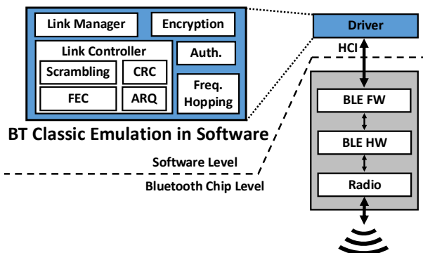
(a) A typical Bluetooth dual-mode chip [5–7] (b) BBC enables Bluetooth Classic on BLE hardware Figure 2: BBC moves entire Bluetooth-Classic processing from HW to SW domain, enabling BLE to support Bluetooth Classic.
