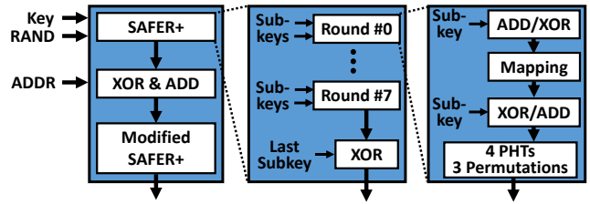
Figure 6: Authentication and Encryption Key Generation
