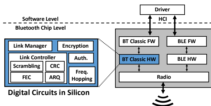
(a) A typical Bluetooth dual-mode chip [5–7] (b) BBC enables Bluetooth Classic on BLE hardware Figure 2: BBC moves entire Bluetooth-Classic processing from HW to SW domain, enabling BLE to support Bluetooth Classic.
