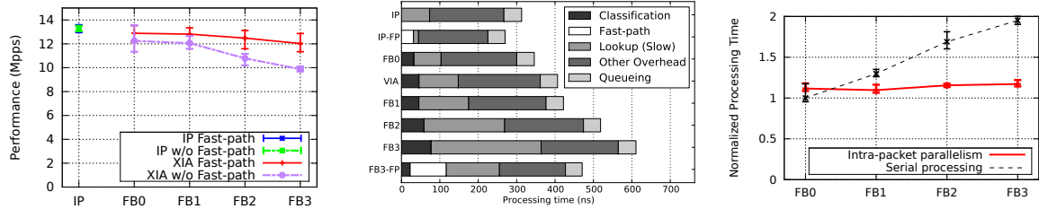
Figure 7: Parallel and serial route lookup cost.
