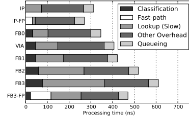
Figure 6: In-memory packet processing benchmark (no I/O).
