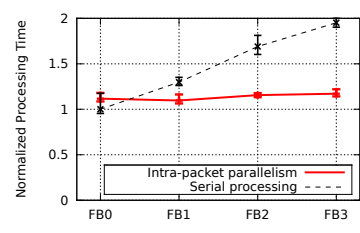
Figure 7: Parallel and serial route lookup cost.
