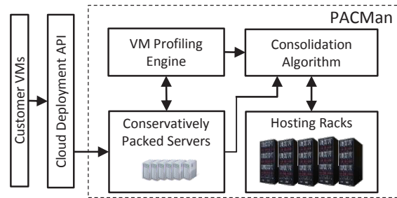
Figure 2: PACMan block diagram.
