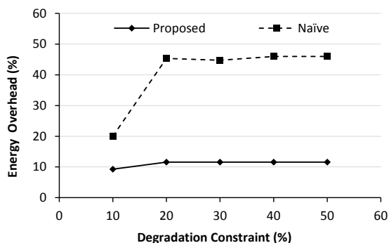
Figure 4: (P-Mode) Excess energy used compared to that used by the optimal solution (computable for a small number of VMs).
